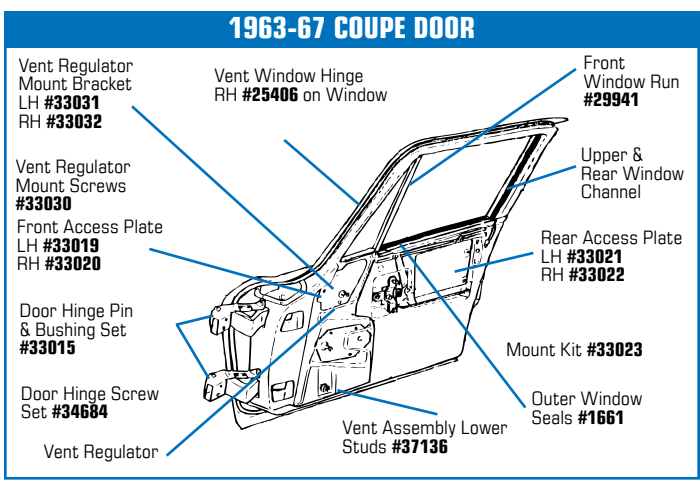
#1736 1963-67 Door Opening Mechanism - LH
