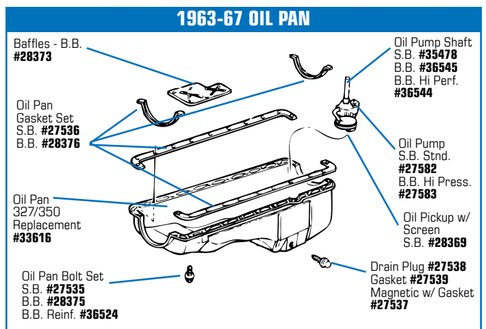
#33616 1963-67 Oil Pan - 327
