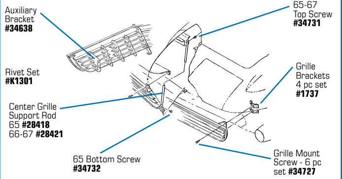
#1751 1965 Grille
