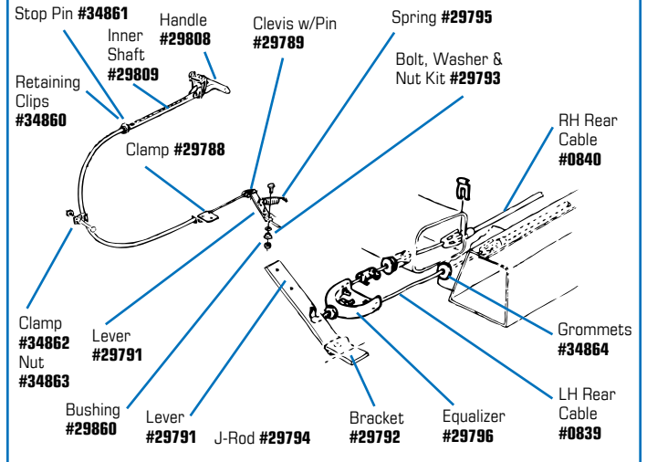
#36369 1965-66 Stainless Steel Park Brake Rebuild Kit
