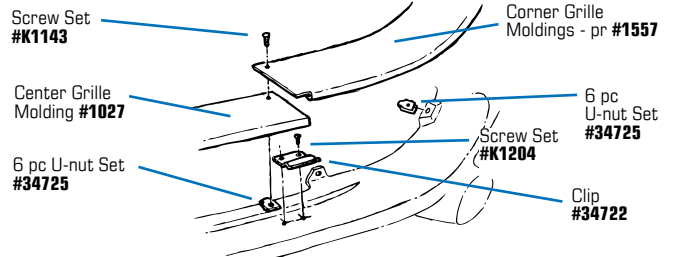
#1745 1963-64 Grille
